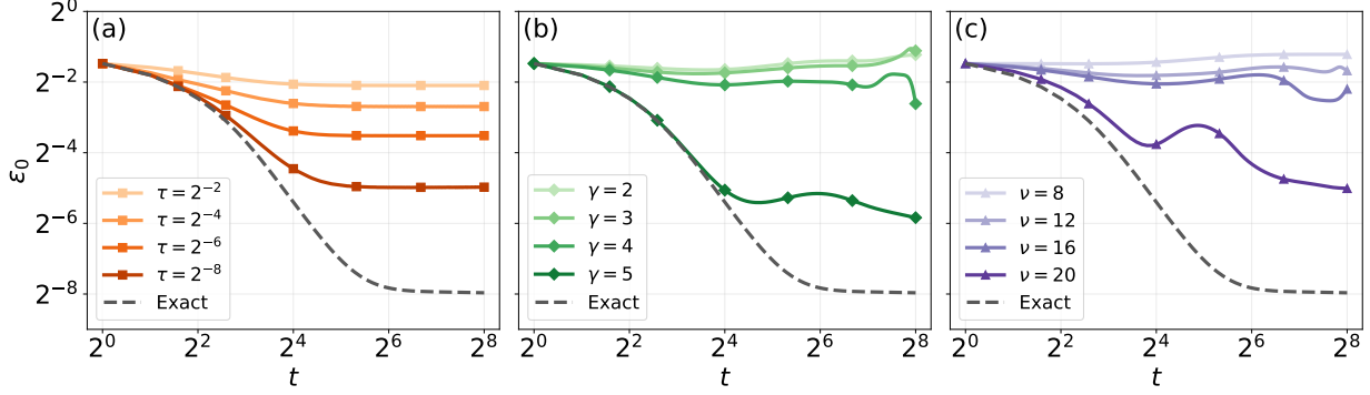
Figure 2: Biased optimization trajectories of Tb-PBS methods. Subplots (a), (b), and (c) show the energy error \epsilon_0 versus the optimization step t of pre-training VQE for the 15-qubit TFIM, which are simulated by using CT-, WT-, and FT-PBS with different truncation thresholds \tau , \gamma , and \nu , respectively. The physical meanings of these thresholds are given in Sec. 3. The dashed curve denotes the exact GD baseline obtained using PennyLane.
