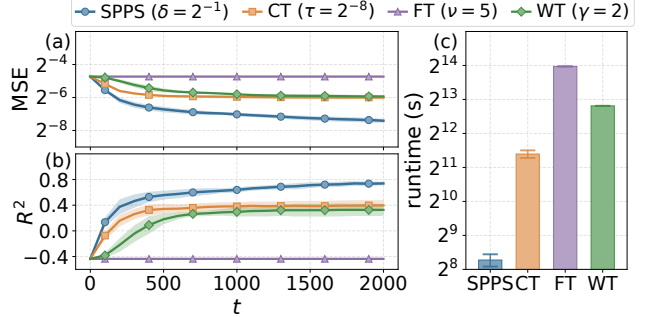
Figure 4: Performance of different PBS methods for pre-training QNN on the 40-QML task. (a,b) Training MSE and test R^2 score versus optimization step t for SPPS, CT-, FT-, and WT-PBS, respectively. (c) Optimization runtime of the four methods. We use \delta = 2^{-1} for SPPS, \tau = 2^{-8} for CT, \nu = 5 for FT, and \gamma = 2 for WT. Error bars show the standard deviation over 5 independent runs.
