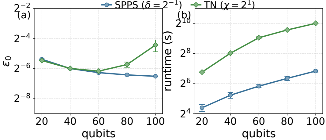
Figure 5: SPPS versus tensor-network simulation on large-qubit VQE pre-training. We compare SPPS and a tensor-network baseline on the L = 6 TFIM VQE benchmark with n \in \{20, 40, 60, 80, 100\} qubits. Figures (a) and (b) report the final normalized energy error \epsilon_0 and the optimization runtime, respectively. Error bars indicate the standard deviation over 10 independent runs.
