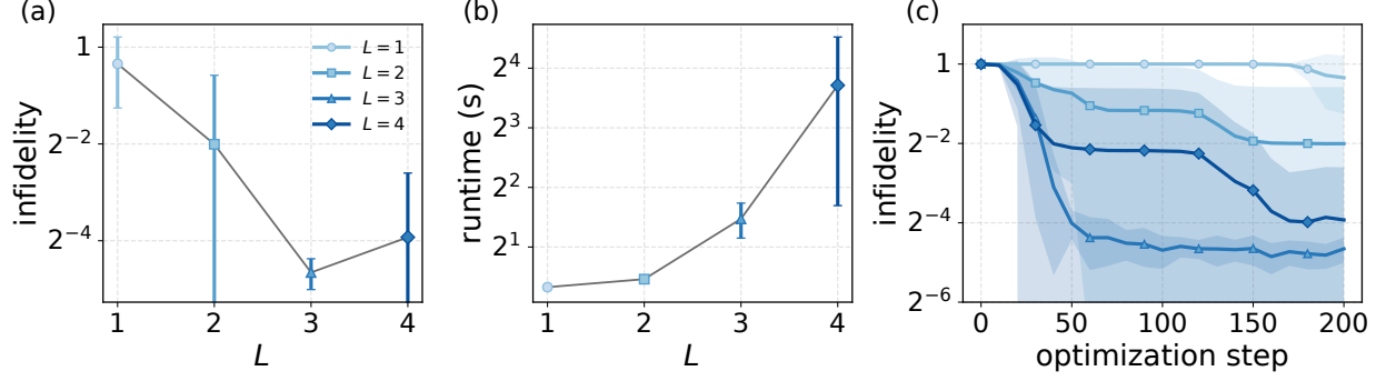
Figure 8: SPPS for preparing MNIST amplitude-encoding circuits. Figures (a) and (b) show the endpoint exact infidelity and cumulative SPPS gradient-estimation runtime, respectively. Figure (c) shows the exact infidelity during optimization. Error bars and shaded regions indicate the standard deviation over 5 MNIST images.
