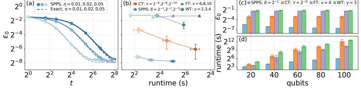
Figure 3: Performance of different PBS methods for pre-training VQE on the TFIM. (a) Energy error \epsilon_0 versus optimization step t for SPPS-driven GD and exact GD on the 15-qubit TFIM with different learning rates. (b) Final energy error \epsilon_0 versus optimization runtime for SPPS and three Tb-PBS methods on the 15-qubit TFIM with different thresholds. (c,d) Final energy error and optimization runtime for system sizes from 20 to 100 qubits. Error bars indicate the standard deviation over 10 independent runs.
