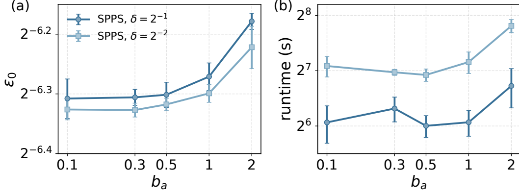
Figure 6: Effect of the sampling-smoothing parameter in SPPS. We evaluate SPPS on the 60-qubit TFIM VQE benchmark with ansatz depth L = 8 and vary the smoothing parameter b_a in the path-sampling distribution. The two figures show the final normalized energy error \epsilon_0 and the optimization runtime. The threshold \delta denotes the adaptive gradient-error proxy tolerance described in App. D.5. Error bars indicate the standard deviation over 5 independent runs.
