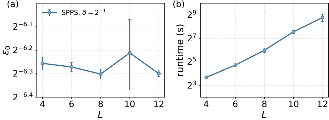
Figure 7: Effect of circuit depth on SPPS-driven VQE pre-training. We evaluate the 60-qubit TFIM VQE benchmark with fixed sampling-smoothing parameter b_a = 0.5 and vary the ansatz depth as L \in \{4, 6, 8, 10, 12\} . The figures report the final normalized energy error \epsilon_0 and the optimization runtime. Error bars indicate the standard deviation over 5 independent runs.
