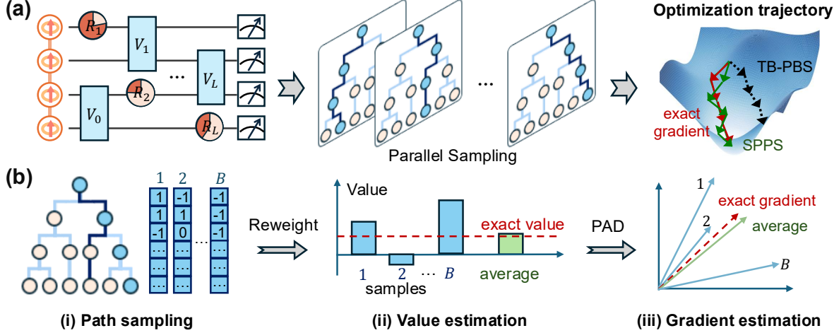
Figure 1: Stochastic Pauli-path simulator for gradient estimation. (a) Overview of the SPSS framework. SPSS samples propagation paths from the full path space and combines them into unbiased estimators of both expectation values and gradients. The sampled paths are generated independently and can therefore be evaluated in parallel. (b) Core algorithm of SPSS. A group of sampled paths is first converted into an unbiased estimator of the target expectation value by importance reweighting. The same path-sampling mechanism is then coupled with path automatic differentiation to obtain unbiased stochastic gradient estimators.
